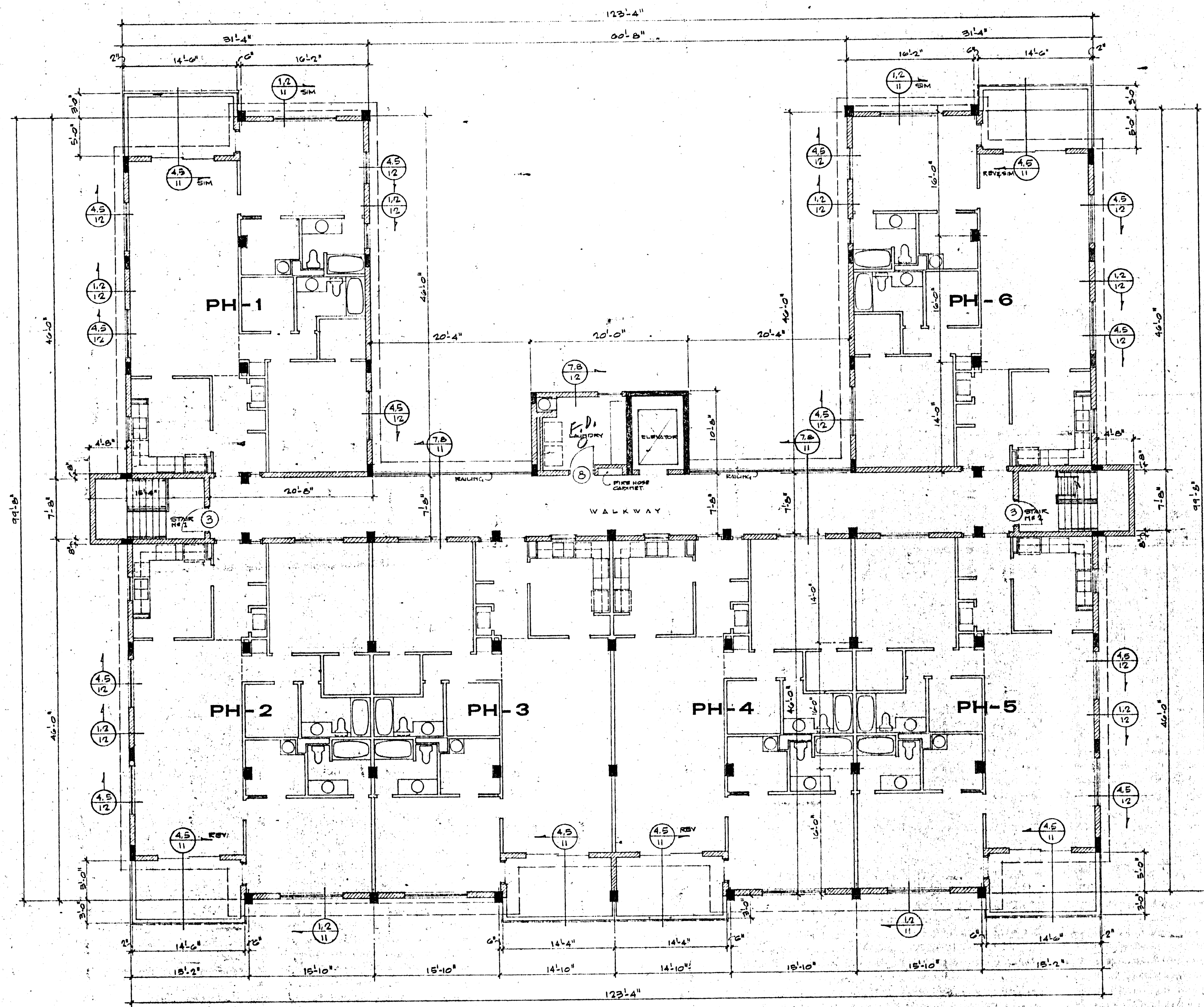
PENTHOUSE FLOOR PLAN scale 1/8" = 1'-0"
