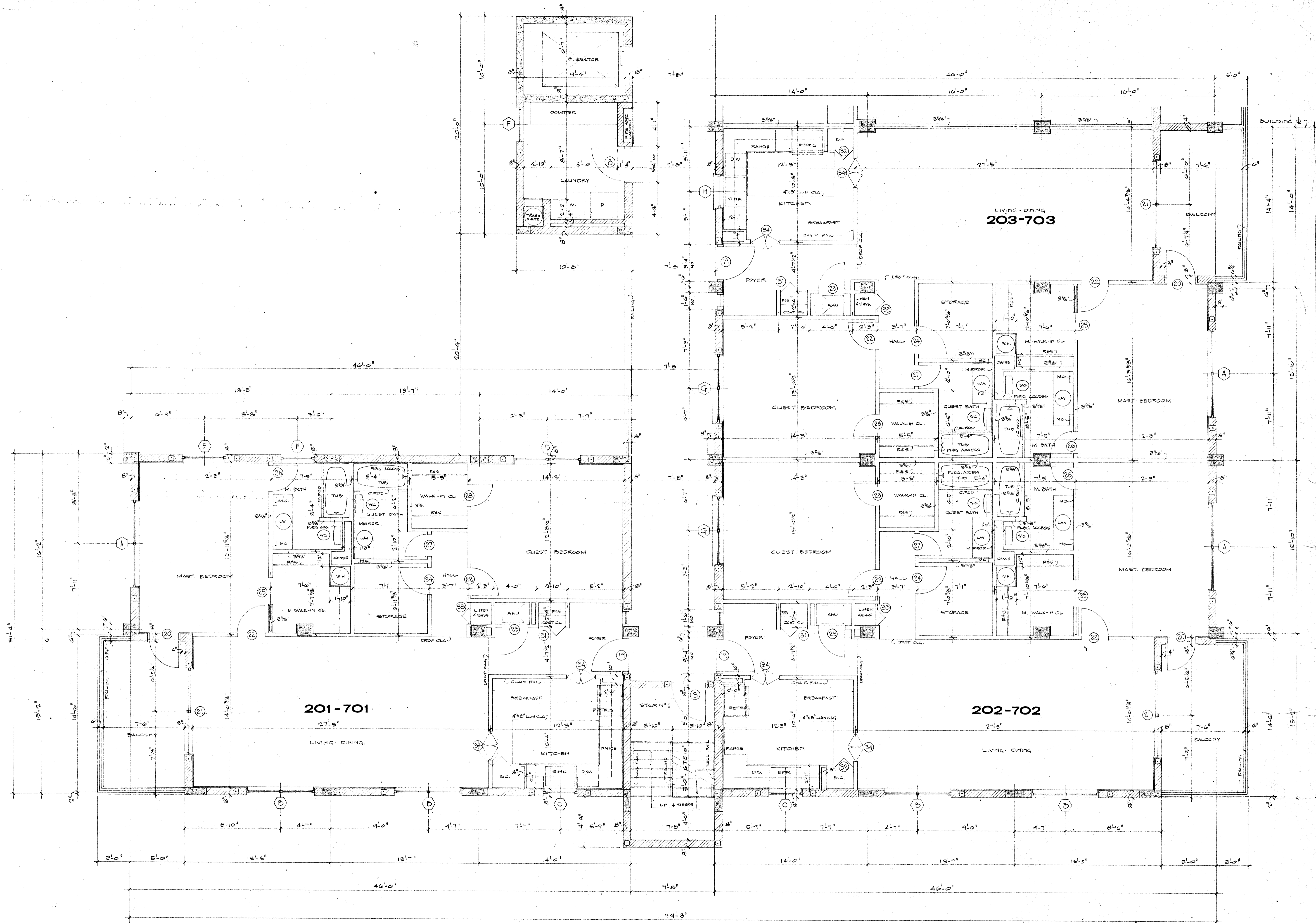
PARTIAL TYPICAL FLOOR PLAN SCALE 1/4" = 1'-0"
