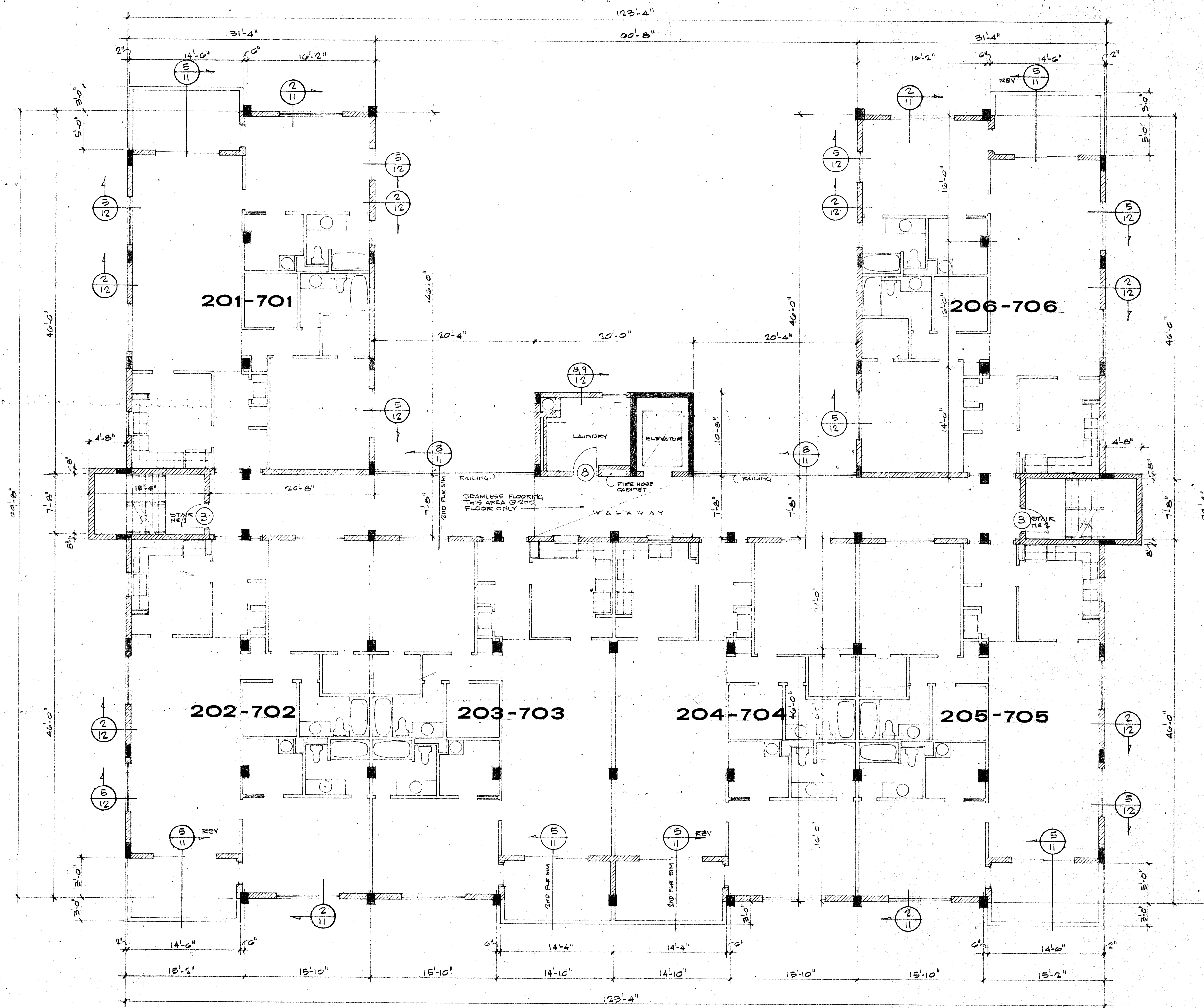
TYPICAL FLOOR PLAN FLOORS 2 THROUGH 7 SCALE 1/8" = 1'-0"
