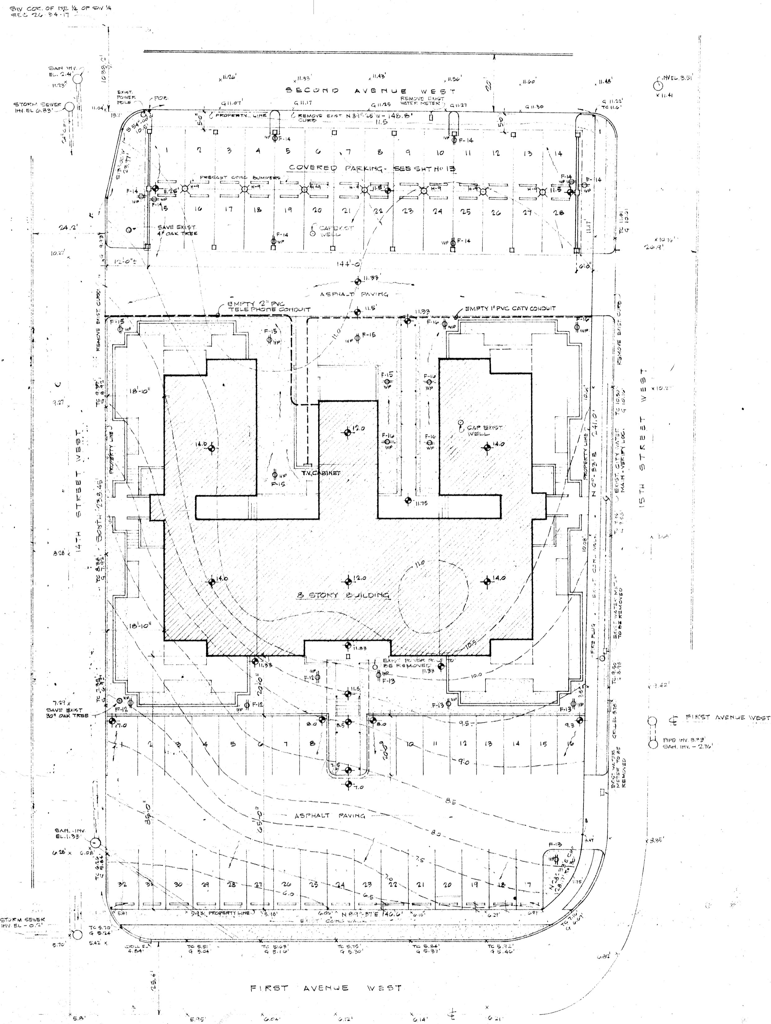
P L O T P L A N SCALE 1" = 20'
