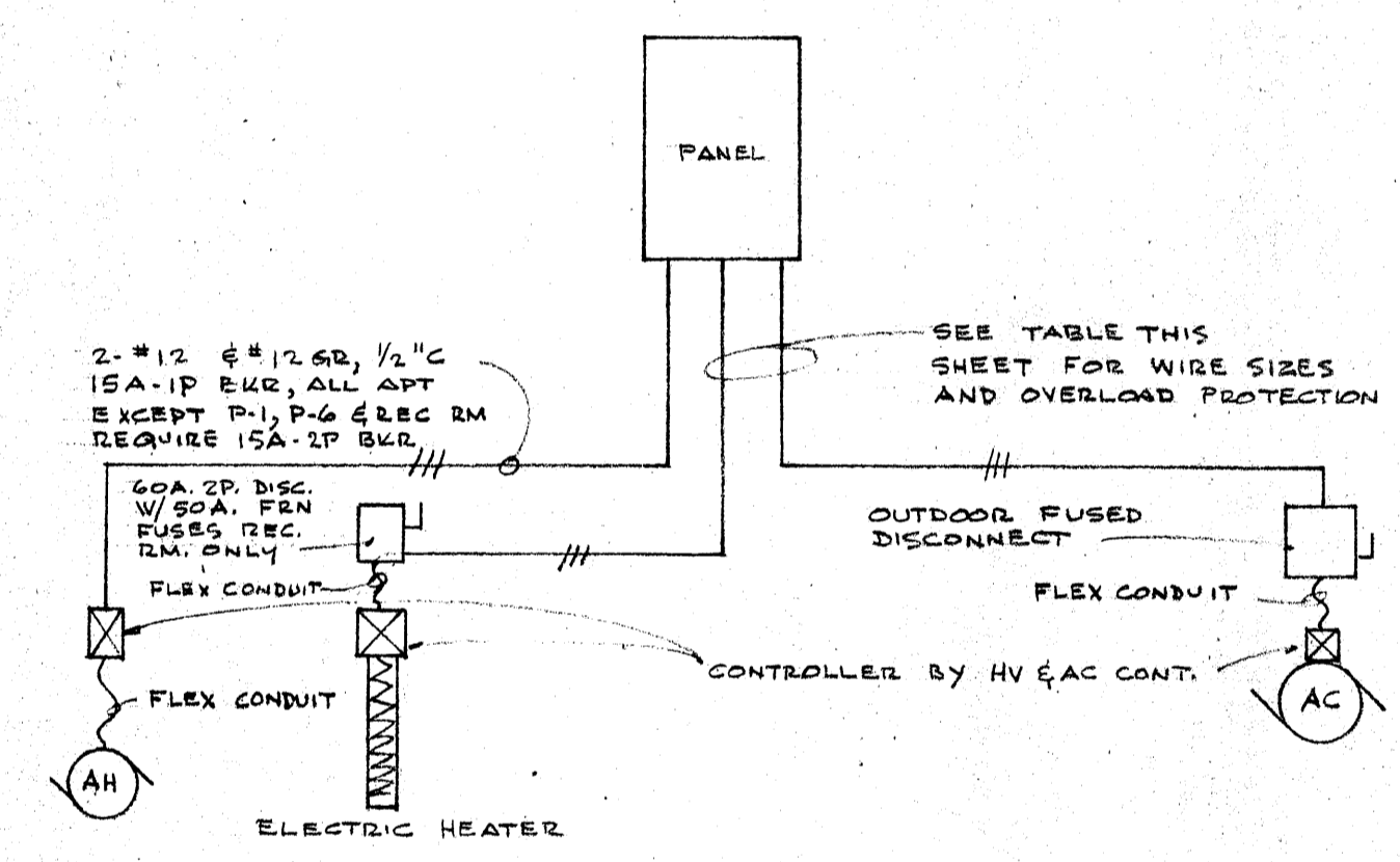
TYPICAL HEATING & AIR CONDITIONING WIRING N.T.S.
