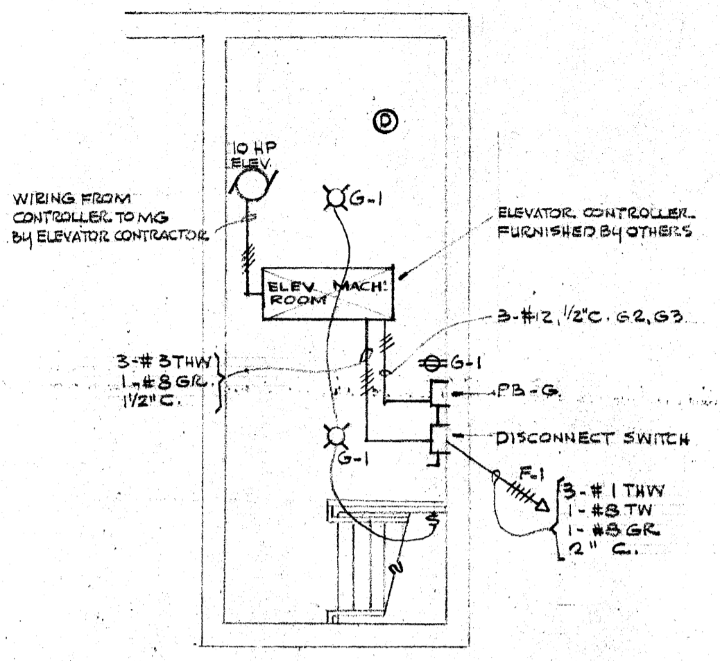
ELEV. MACH. ROOM SCALE 1/4" = 1'-0"
