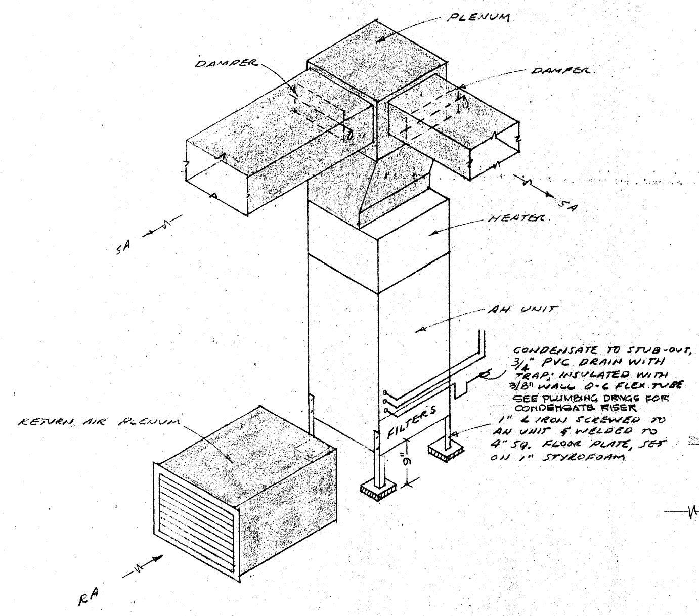
TYPICAL AH UNIT DETAIL SCALE 1/2" = 1 FT
