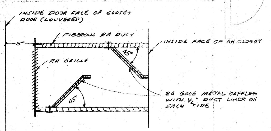
RETURN AIR DUCT DETAIL SCALE 1" = 1 FT
