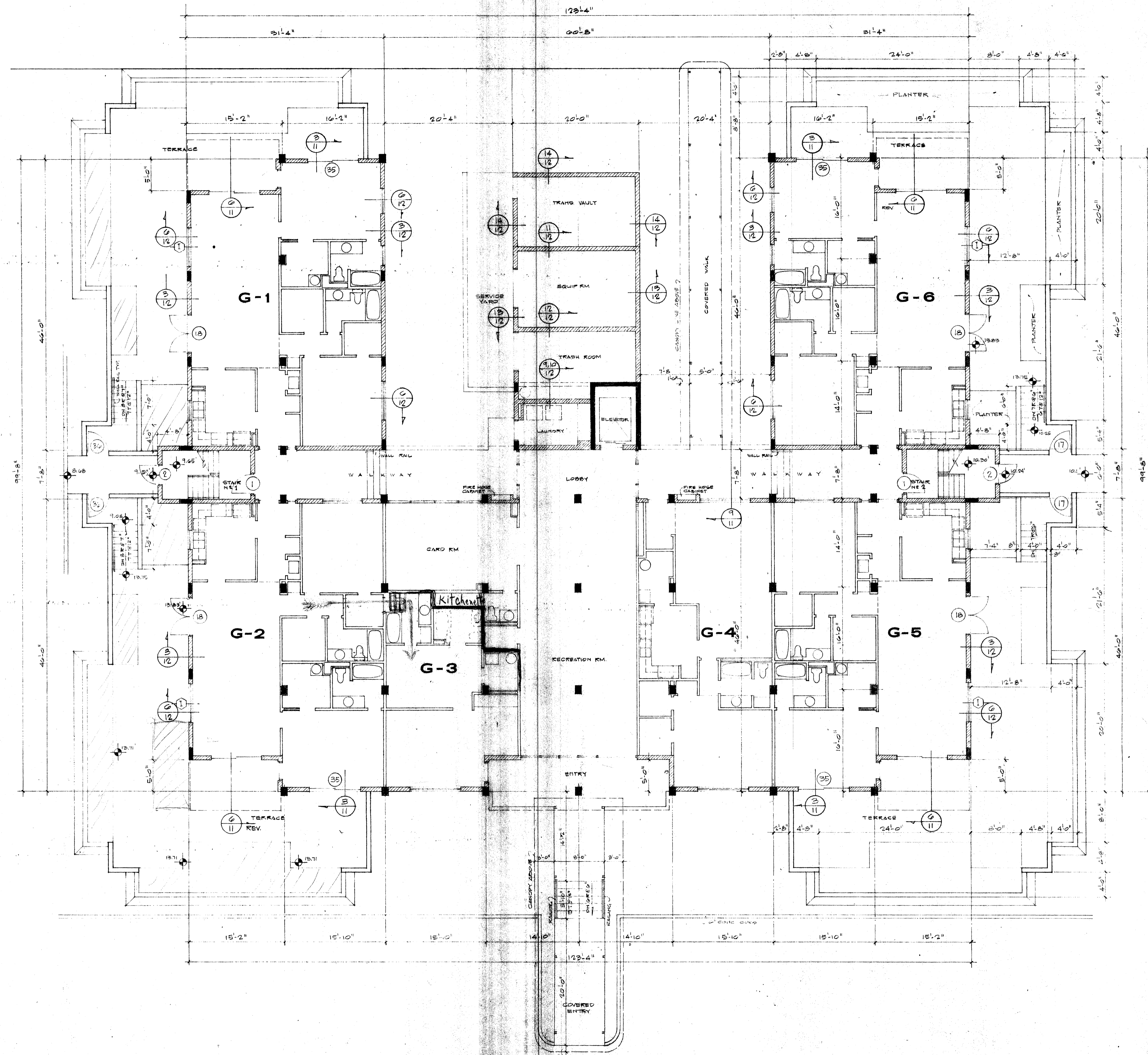
G R O U N D F L O O R P L A N SCALE 1/8" = 1'-0"
