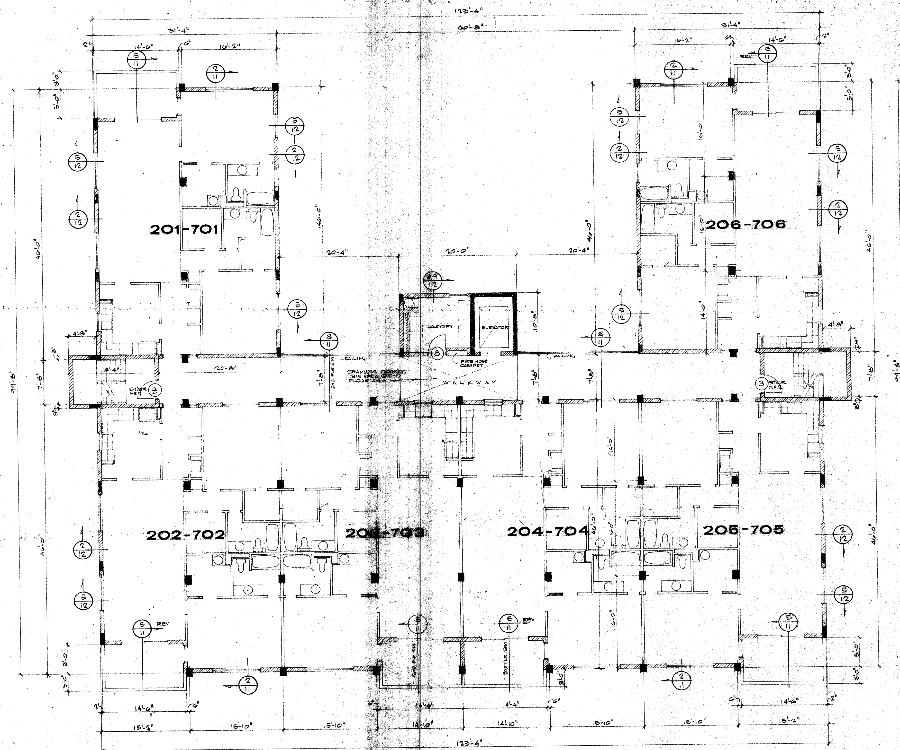
TYPICAL FLOOR PLAN FLOORS 2 THROUGH 7 SCALE 1/8" = 1'-0"
