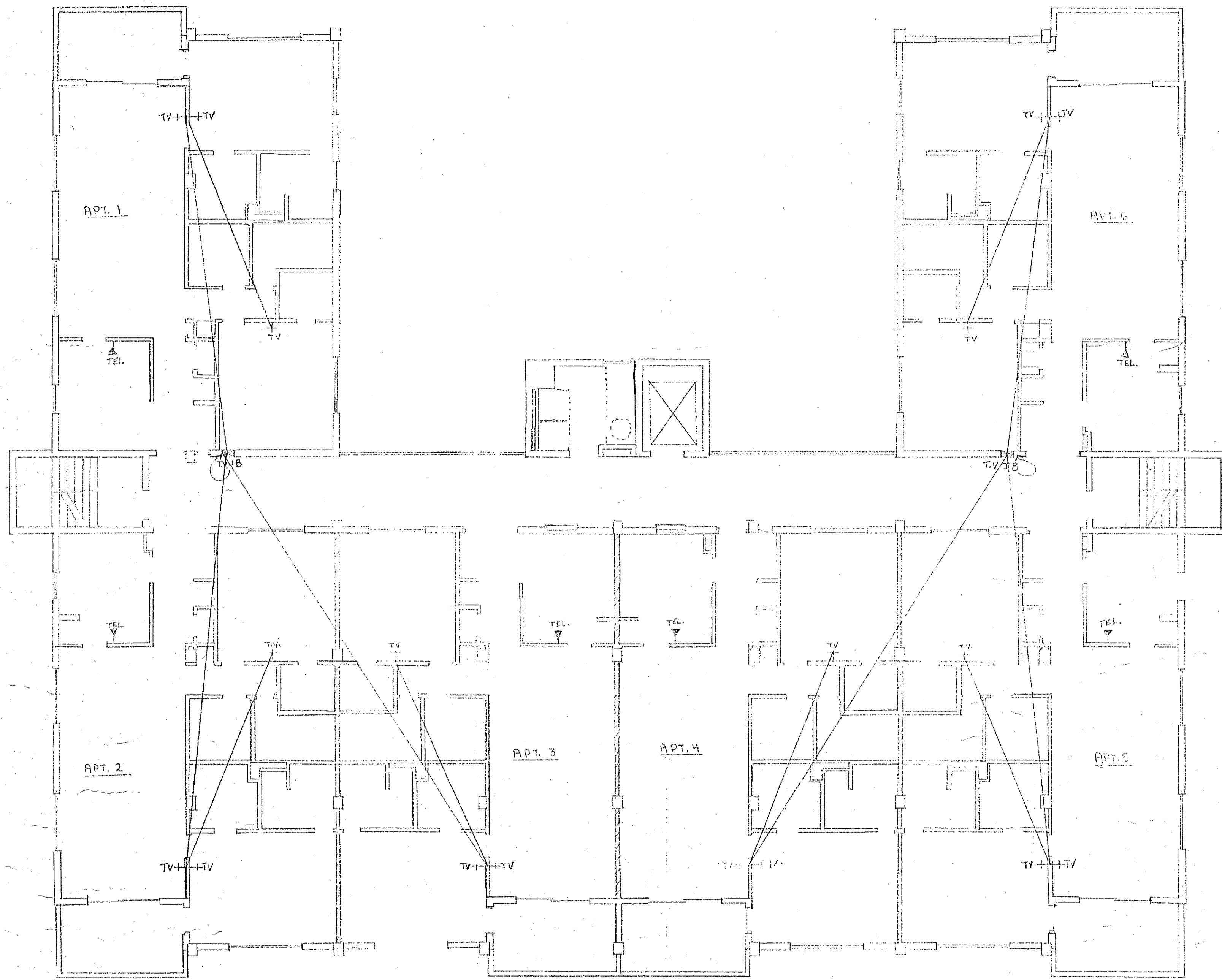
TYPICAL FLOOR ELECTRICAL PLAN FLOORS 2 THROUGH 7 - 3RD FLOOR SHOWN SCALE 1/8" = 1'-0"
